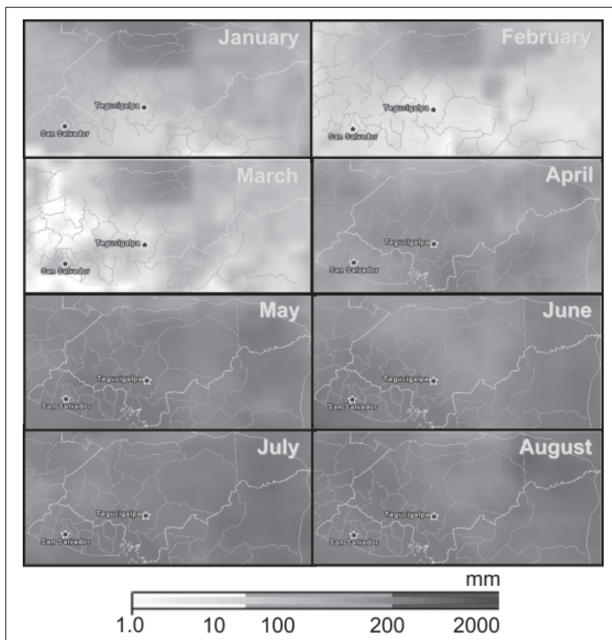
Figure 3. Rain patterns maps from the TRMM satellite for Honduras during January to August 2010 (NEO/NASA)
